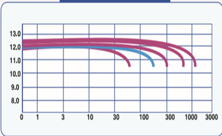
Discharging Characteristics
