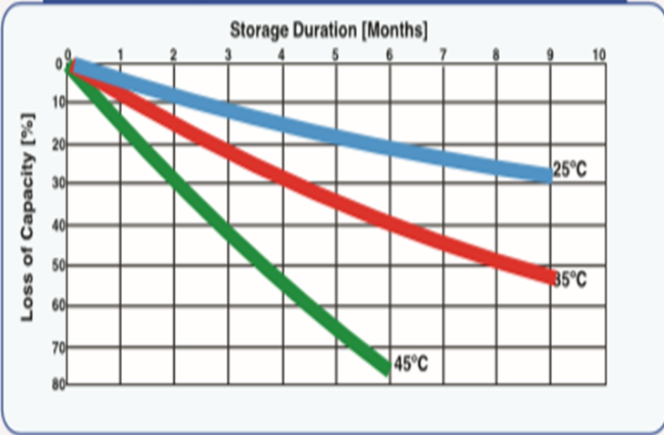
Self Discharge Characteristics - Tubular Batteries
