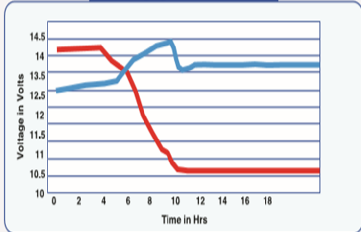
Charging Characteristics
