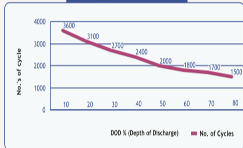
Cycle Life Vs DOD
